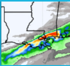
PRECIPITATION FORECASTS
